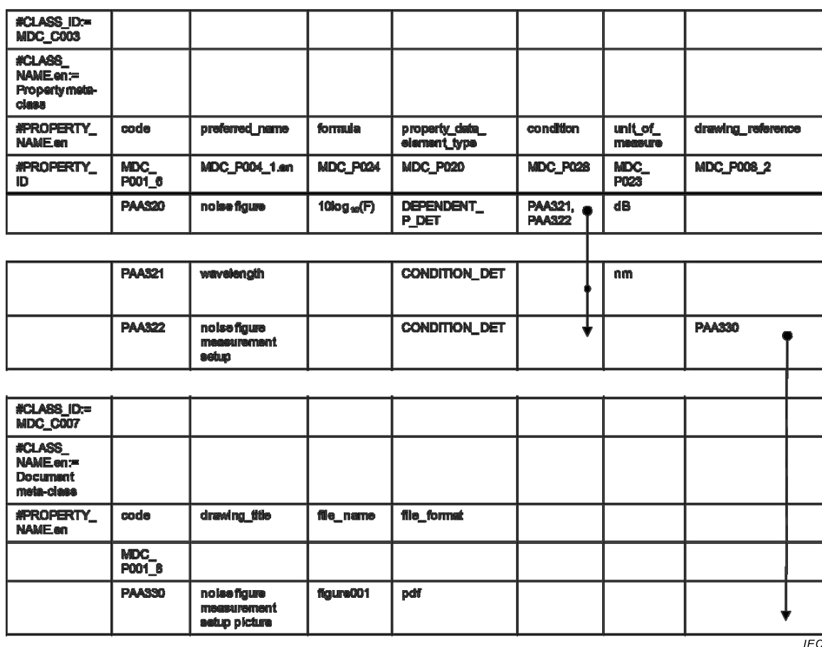
Figure 30 – Implementation in IEC 62656-1 spreadsheet format of the example in Figure 29
