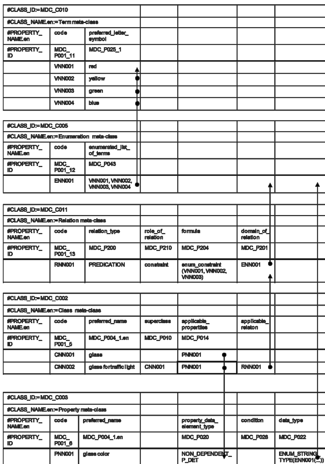
Figure 40 – Example – Restricted enumeration (IEC 62656-1 spreadsheet format)
