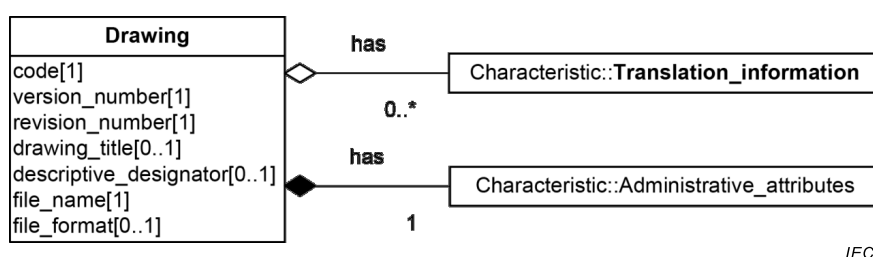
Figure 17 – Drawing (UML class diagram)
